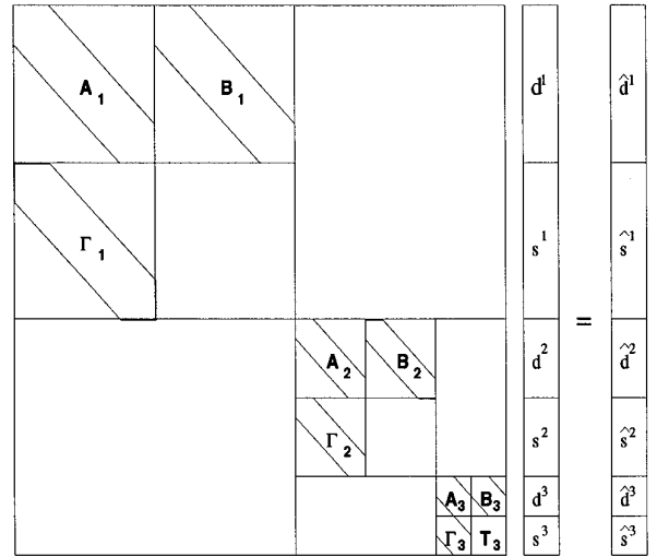
FIG. 22. Illustration of the application of the nonstandard form to a vector.
