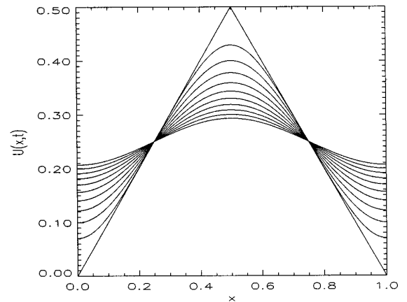
FIG. 4. Solution of the heat equation using the NS-form of the exponential with \Delta t = \Delta x = 2^{-9} and \nu = 1.0 , i.e., Eq. (5.14).
