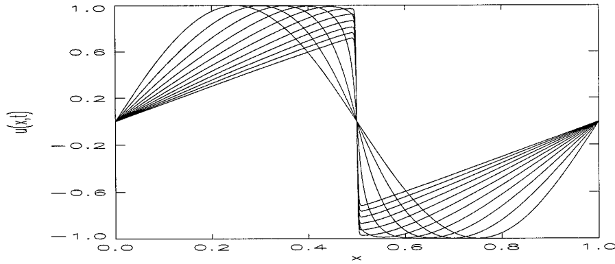
FIG. 7. The projection on \mathbf{V}_0 of the solution of Burgers' equation at various time steps computed via the iteration (5.21). In this experiment n = 15, J = 9, \Delta t = 0.001, \nu = 0.001, and \varepsilon = 10^{-6} . This figure corresponds to Example 1 of the text.
