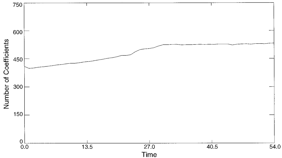
FIG. 16. The total number of significant wavelet coefficients per time step. This figure corresponds to Example 4 of the text.
