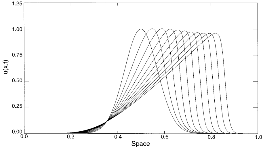
FIG. 15. The projection on V_0 of the solution of (5.27) at various time steps. In this experiment n = 15, J = 4, \Delta t = 0.001, \varepsilon = 10^{-6} , and \nu = 0.005 . This figure corresponds to Example 4 of the text.
