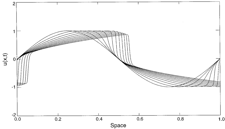
FIG. 19. The projection on \mathbf{V}_0 of the solution of cubic Burgers' equation (5.30) at various time steps, computed using a sinusoidal initial condition. In this experiment n = 13, J = 6, \Delta t = 0.001, \nu = 0.001, and \varepsilon = 10^{-6} . This figure corresponds to Example 5 of the text.
