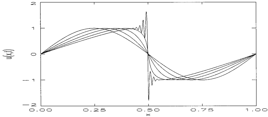
FIG. 9. The projection on \mathbf{V}_0 of the solution of Burgers' equation at various time steps computed via the iteration (5.21). In this experiment n = 10, J = 4, \Delta t = 0.001, \nu = 0.001, and \varepsilon = 10^{-6} . An analogue of the Gibbs phenomenon begins because the shock cannot be accurately represented by n = 10 scales. Observe that the scheme remains stable in spite of the oscillations. This figure corresponds to Example 2 of the text.
